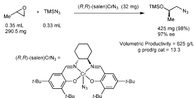
Scheme 32. Kinetic resolution of propylene oxide by ring opening with TMSN 3
