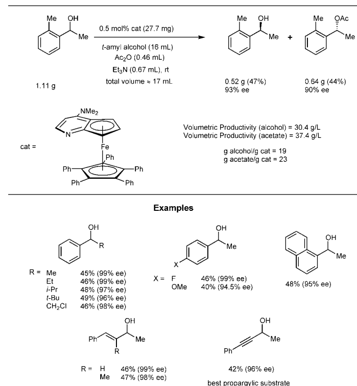
Scheme 5. Fu's kinetic resolution of secondary alcohols
