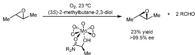
Scheme 19. Schurig's oxidative kinetic resolution of epoxides
