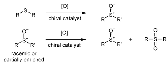
Scheme 13. Enantioselective synthesis and kinetic resolution of sulfoxides
